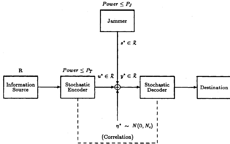
Fig. 1. Gaussian arbitrarily varying channel.
