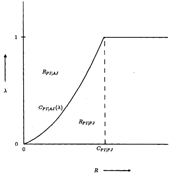
Fig. 2. Achievable regions for GAVC PI/PJ and PI/AJ.
